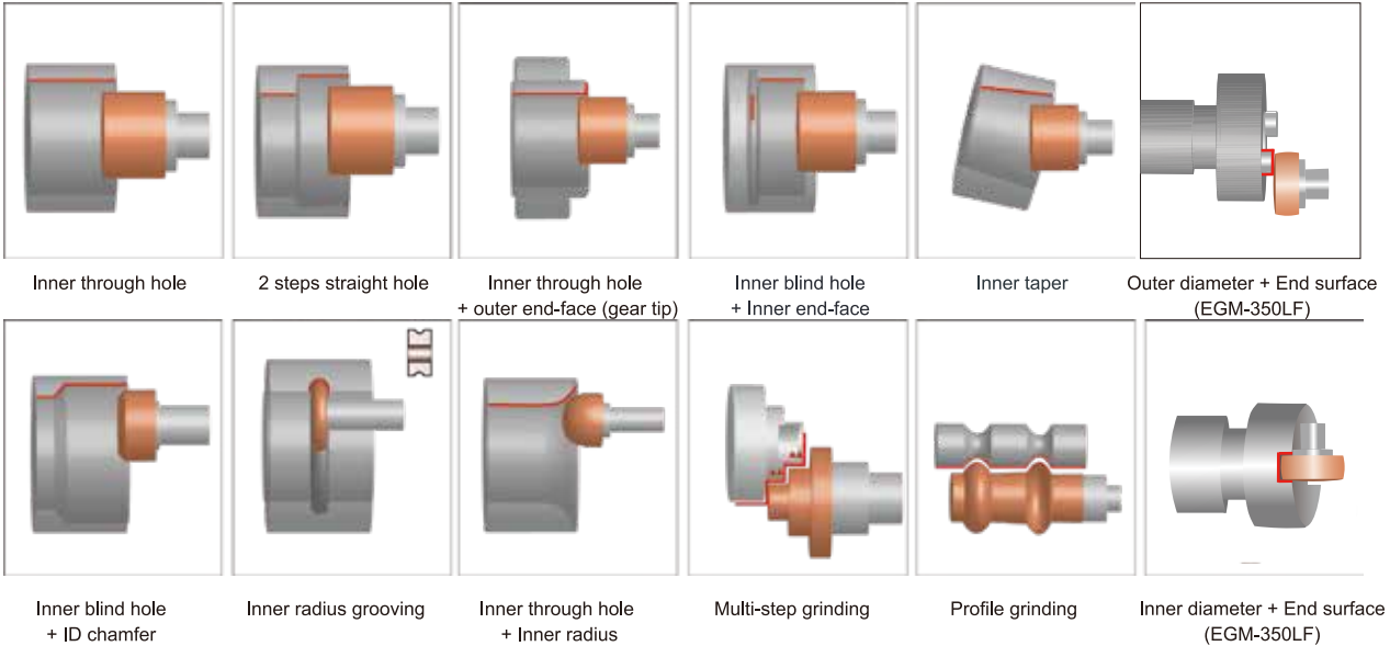
Standard grinding cycles and multi-steps graphic conversational functions.
